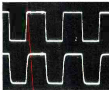
Fig. 5. 7500 Hz input and output for system with flat response to 50 kHz and a 10 dB roll-off at 100 kHz. Note that with the exception of some slight rounding, the waveform is intact.
