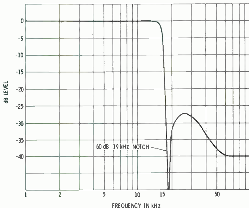
Fig. 2 Frequency response of a 15 kHz low pass filter with 19 kHz notch.
