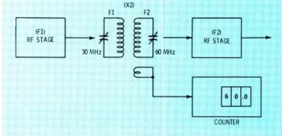
Fig. 4 Use tight coupling to the secondary of the RF transformer in a multiplier circuit.
