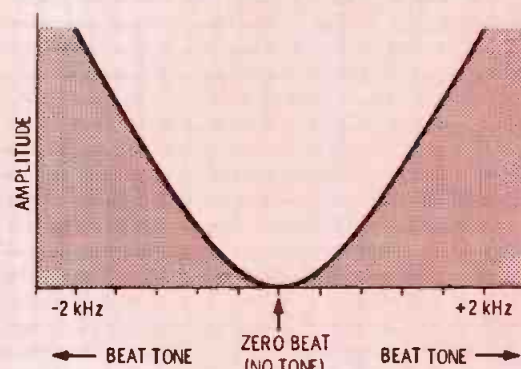
Fig. 2B When the counter frequency is above or below WWV, a beat tone will be heard. The objective is zero tone in the center.
