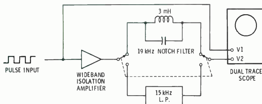
Fig. 3 This is a simplified diagram of a test setup to check the affect of 19 kHz notch and 15 kHz low pass filters on transient response.
