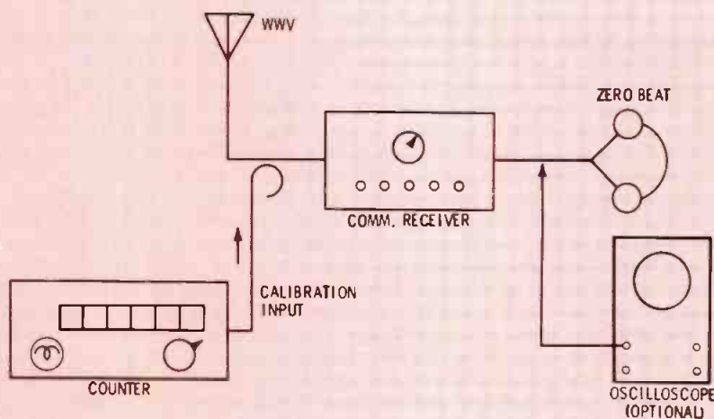
Fig. 2a The setup for calibration against WWV. Listen for a zero beat in the phones. The scope also can be used to detect a more exact null.
