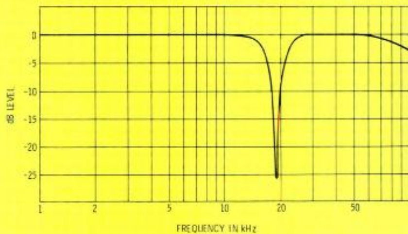
Fig. 1 Frequency response of a 19 kHz notch circuit.
