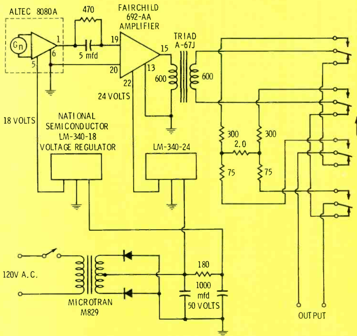
Fig. 1 This is the schematic for the pink noise generator.
