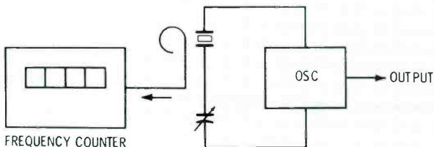
Fig. 5 When testing a crystal oscillator, couple close to the crystal itself. Then you can determine the actual frequency. When some counters indicate digits are in the overflow circuitry, the readouts will give a reading of digits after the decimal, adding to the unit's capability.
