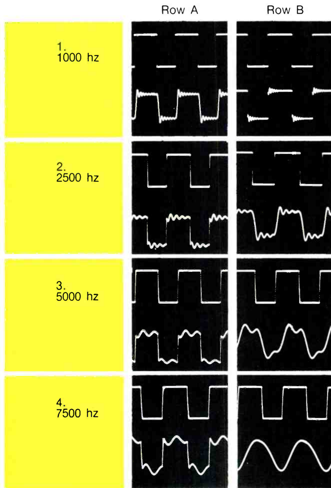
Fig. 4. These dual trace photos illustrate the waveform distortion that can be expected from each type of filter circuit. In each case, the top trace is the input signal and the bottom trace is filter output. Row "A" is for the 19 KHZ notch circuit and row "B" is for the 15 KHZ low pass filter which also includes a very sharp 19 KHZ notch. Input frequencies are as follows: 1. 1000 hz, 2. 2500 hz, 3. 5000 hz and 4. 7500 hz. The higher frequency traces have been expanded to the same scale as the 1000 hz traces so that comparisons can more readily be made.
