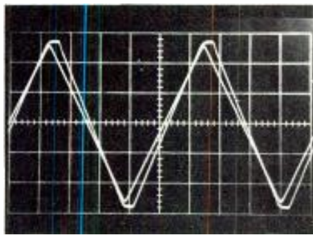
Fig. 2 Checking clipping and overload recovery time. Full power, undistorted 20 kHz triangle wave (lower level trace); clipped triangle with fast recovery. Scales are 20V/cm vertical, 10 us/cm horizontal.
