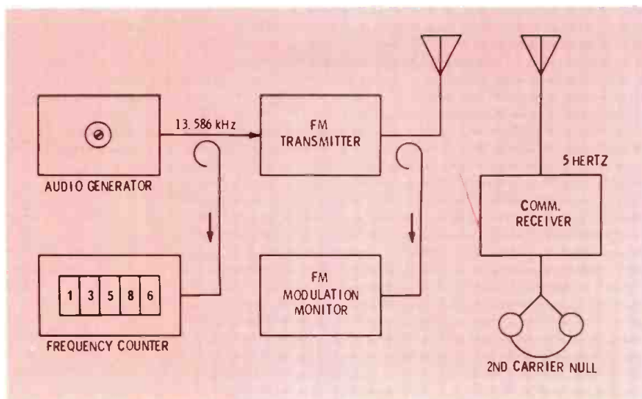
Fig. 3 Setup for calibration of FM modulation monitor. Measure the audio frequency so that it is exact.
